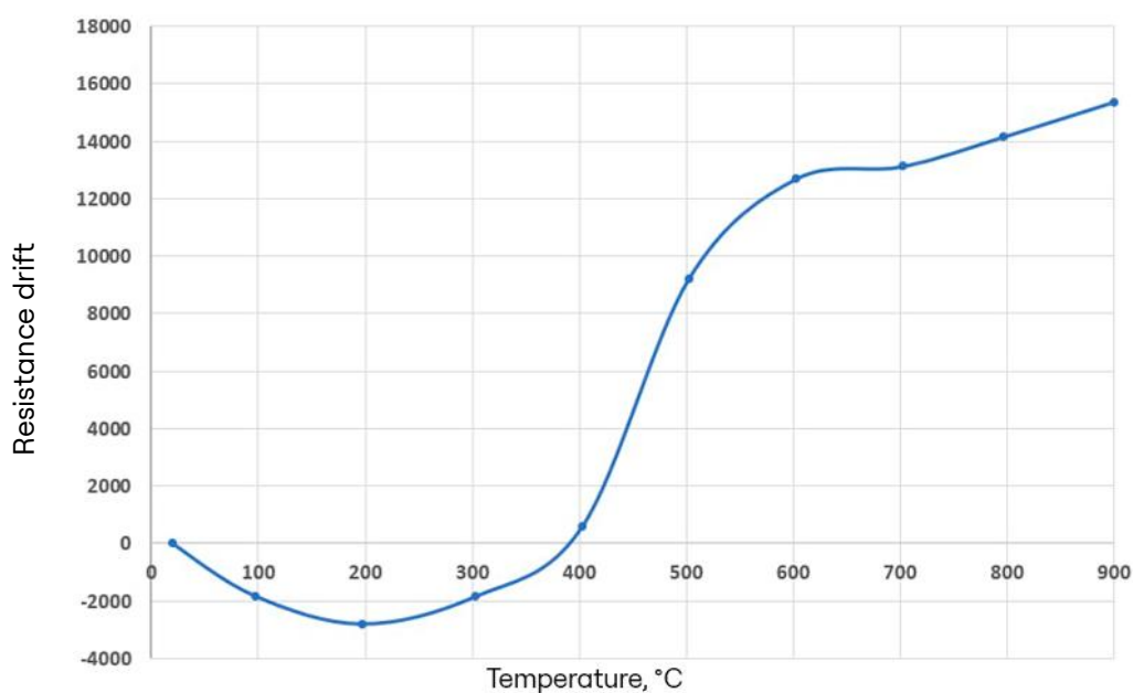
Diagram 2. Resistance drift due to the temperature**
